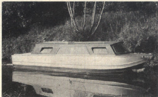
30 ft. x 6 ft. 10 in. stern cockpit. 6 berth. Complete fully fitted. Inboard or outboard engine. £1,850 excluding engine
